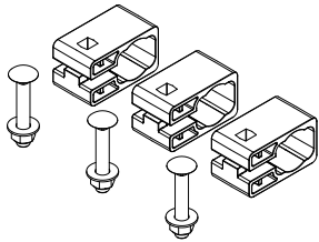
(3) Clamp sets: clamp bolt washer nylok nut
